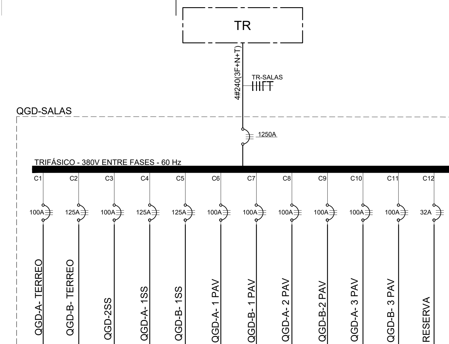
DIAGRAMA UNIFILAR QGD SALAS
